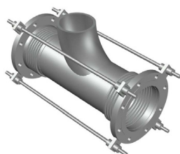
Pressure balanced compensator
