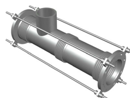
Universal pressure balanced compensator
